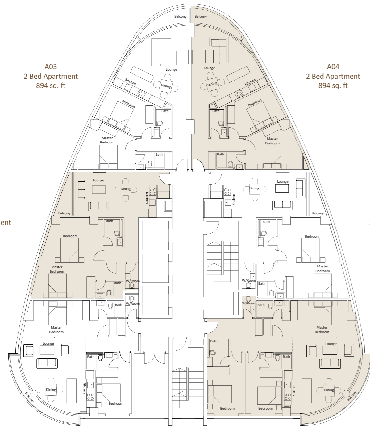
Tower One: 1st Floor Plan
