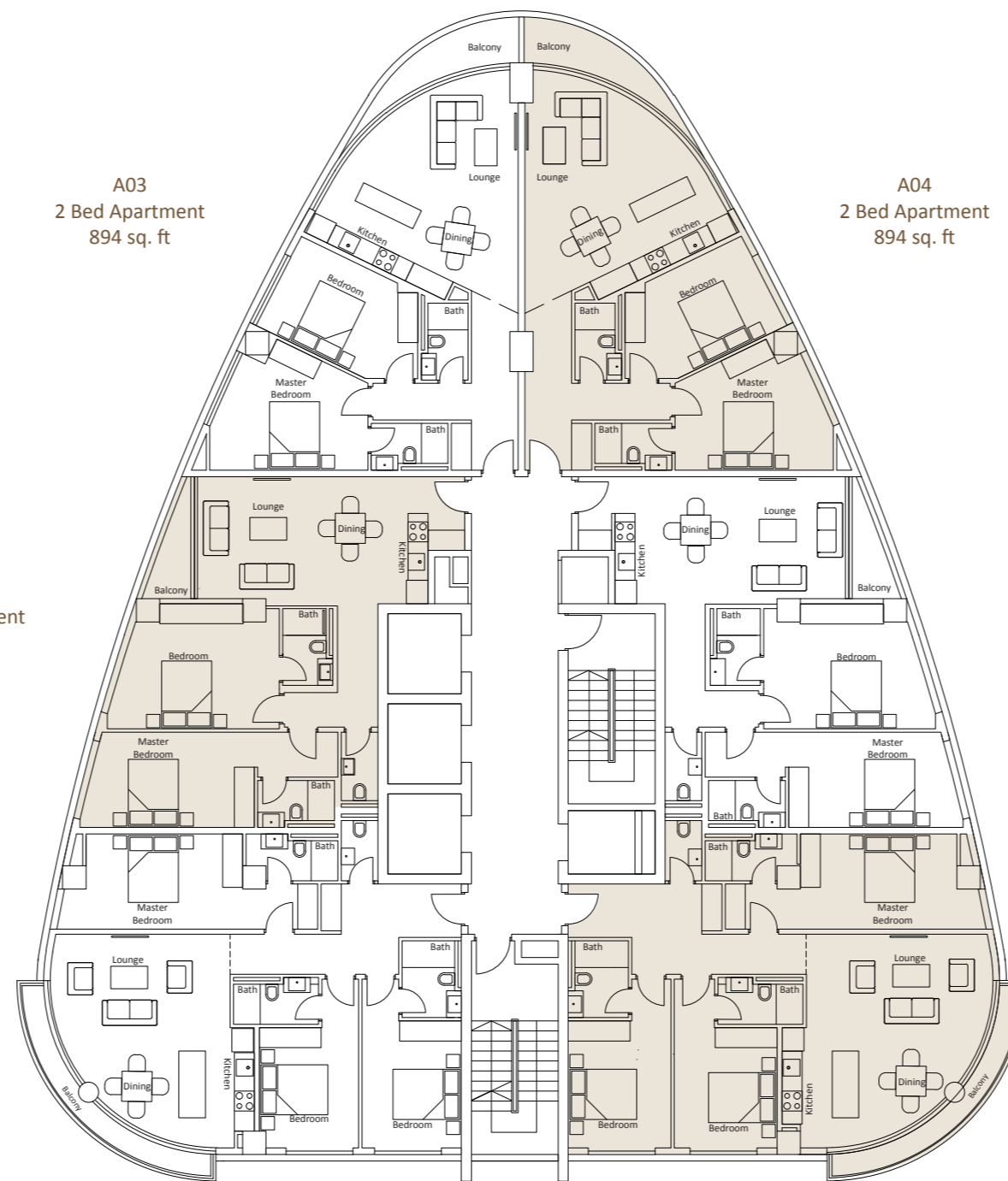
Tower One: 2nd - 8th Floor Plan
